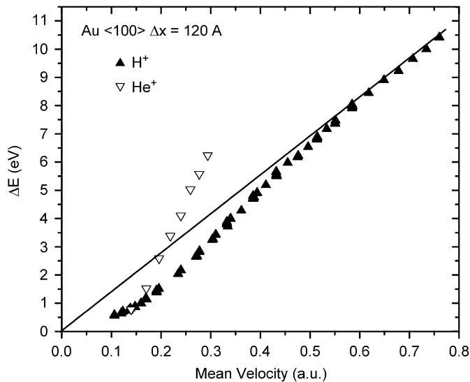
Fig. 1. Energy loss of protons and helium ions transmitted through the (100) direction of a single crystal gold thin foil of 120 Å.
